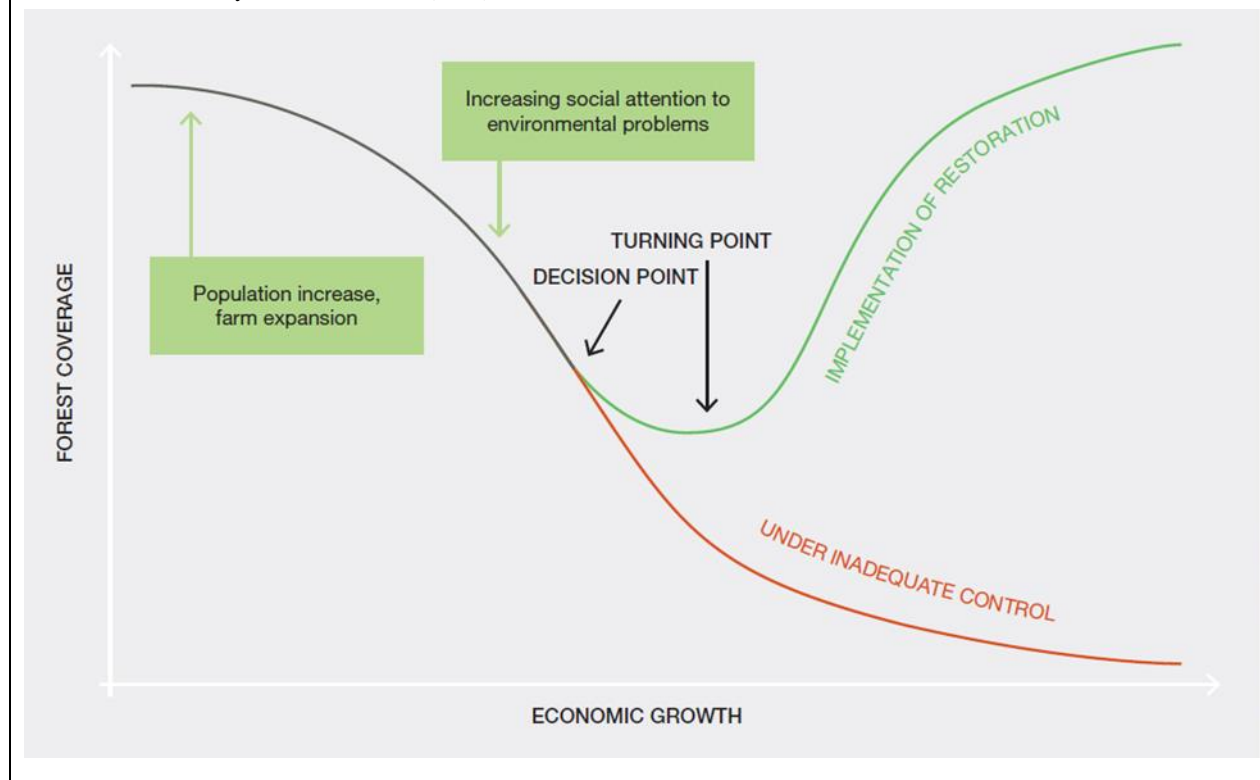
Figure SPM.3
