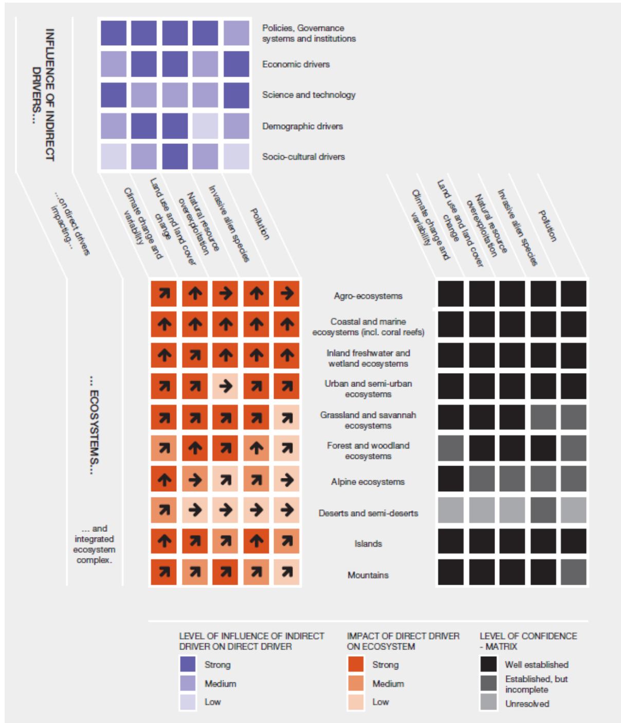
Figure SPM.7
