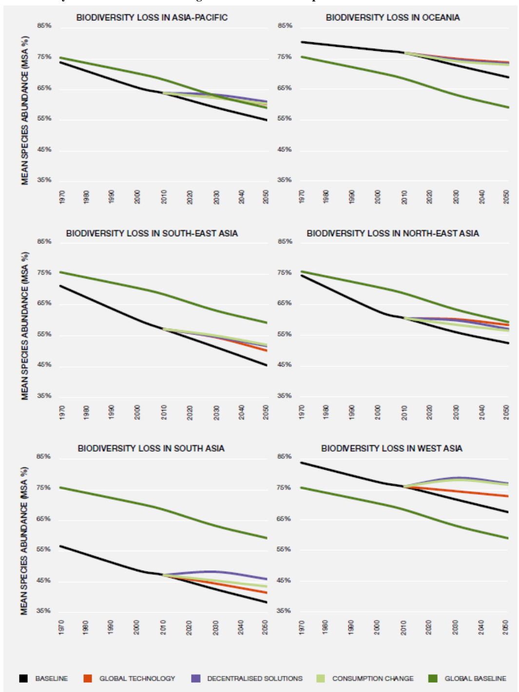
Figure SPM.9
